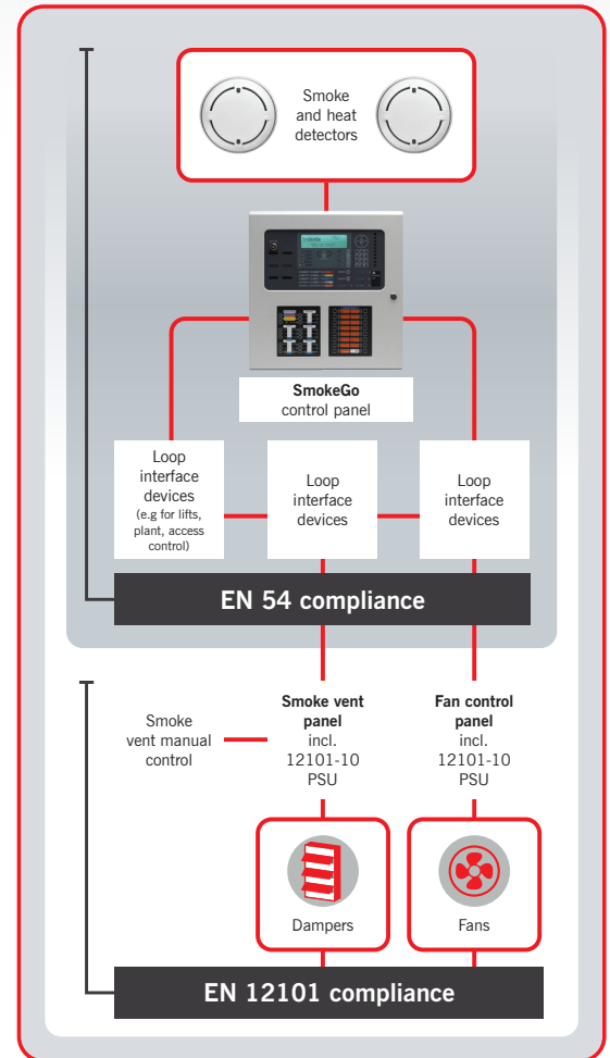
Typical SmokeGo setup
